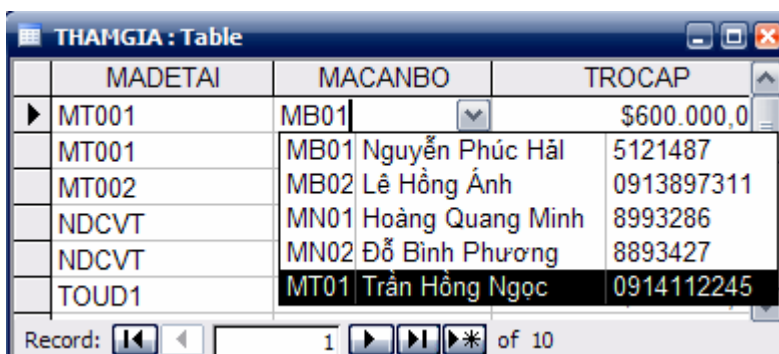
Lookup cho Field MaCanBo
