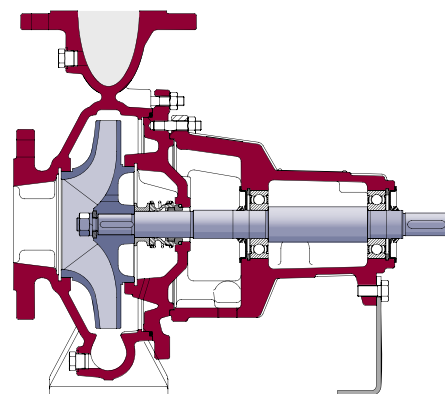
Fig. 1.1.12: Standard pump with single-suction impeller
