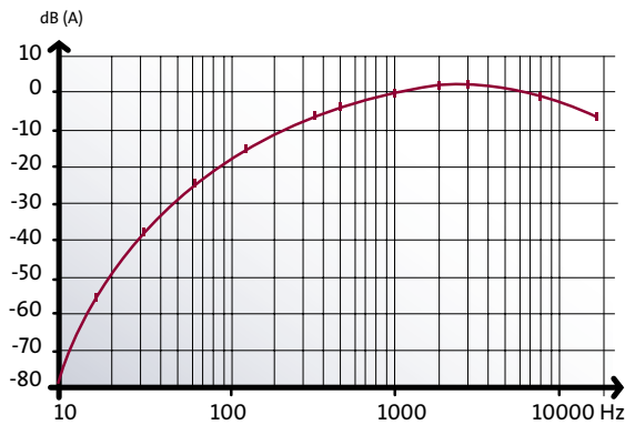
Fig. 2.1.16 A-weighting curve
