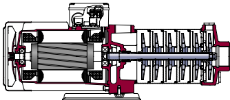
Fig. 1.1.24: Horizontal multistage end-suction pump
