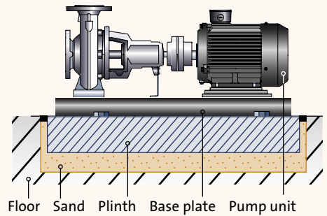
Fig. 2.1.8: Floating plinth
