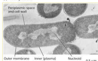
(a) Prokaryotic cell
