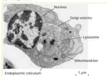
(b) Eukaryotic cell
