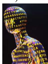
Human Genome Project
