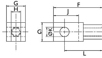
Fork Clevis
