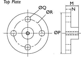
Top Plate
